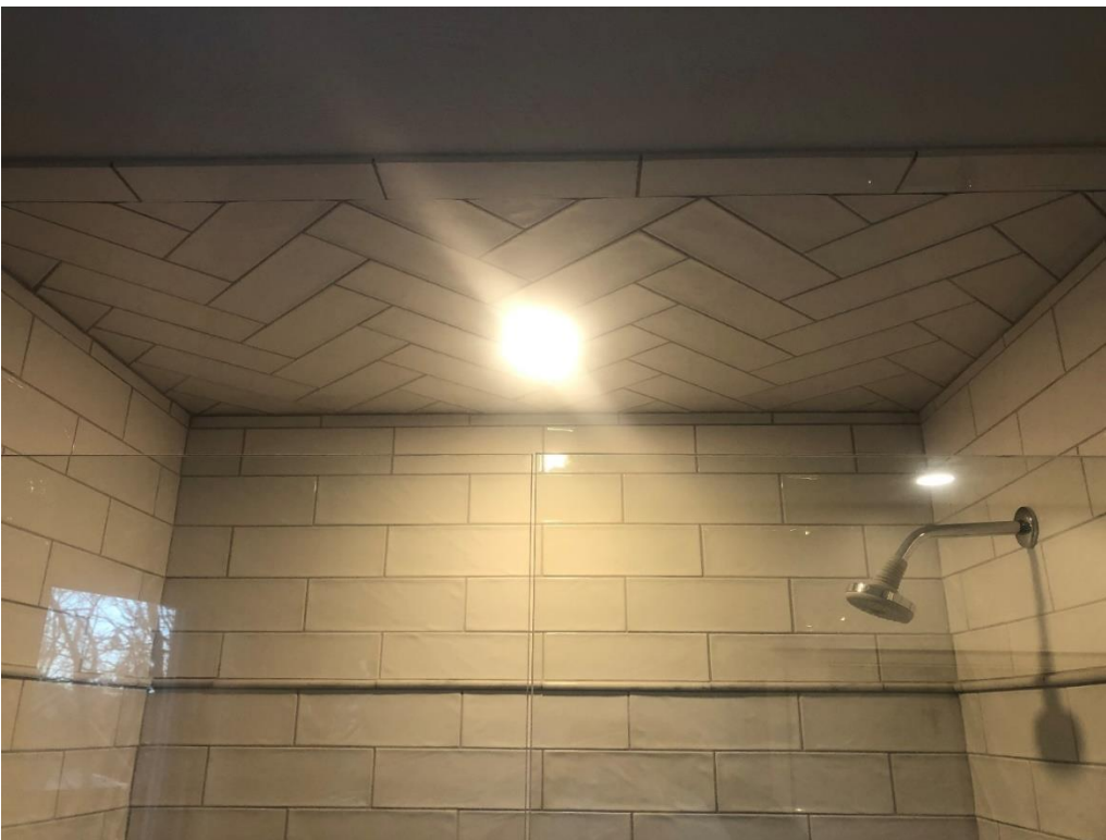
Herringbone ceiling bonnet with bullnose edge, pencil accent molding and a DALI wet installation area light.
